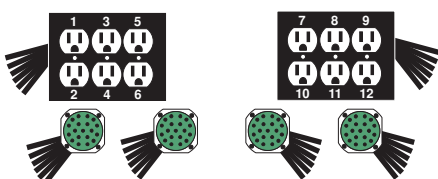
(DRSW362) All Connectors wired separately (36ch)
