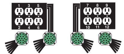
(DRSW362) Both Edison set hardwired to Soca (24ch)
