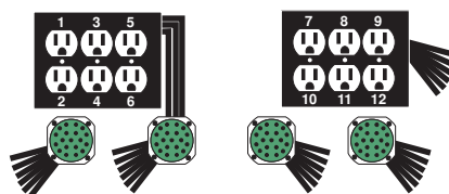
(DRSW362) One Edison set hardwired to Soca (30ch)
